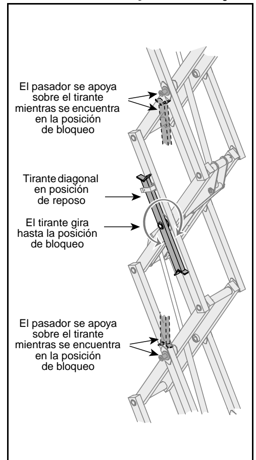
Figure 8: Tirante diagonal
